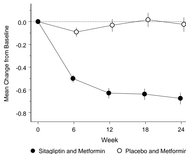
Figure 2 Mean Change from Baseline for HbA_{1c} (%) over 24 Weeks with Sitagliptin 100 mg – Total Daily Dose added to Metformin ( \geq 1500 mg) or Placebo added to Metformin ( \geq 1500 mg) in Patients with Type 2 Diabetes †‡
