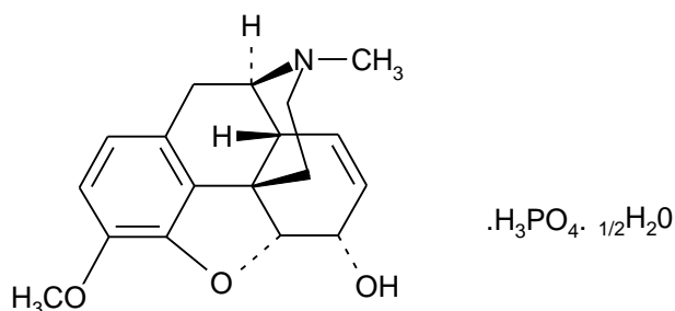
Codeine phosphate hemihydrate MW 406.37
