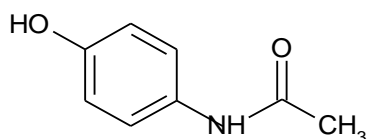
Paracetamol MW 151.17
