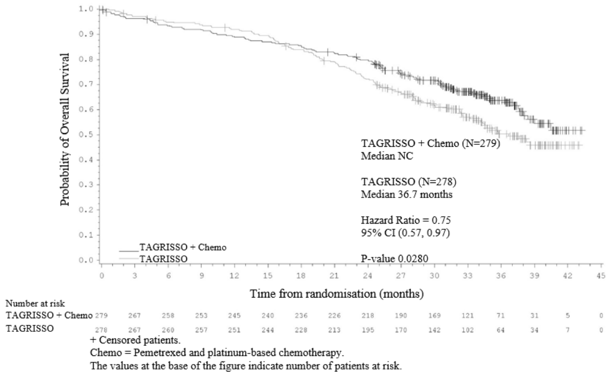
Figure 8 Kaplan-Meier Curves of Overall Survival in FLAURA2
