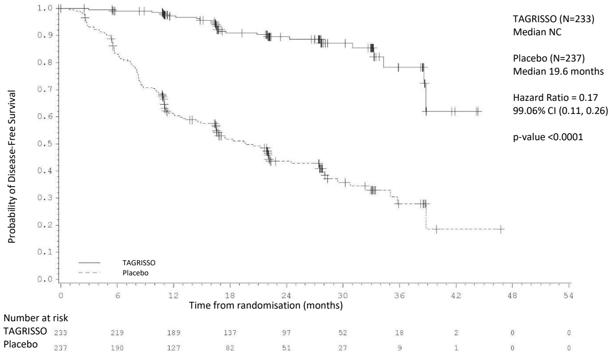
Figure 1 Kaplan-Meier curve of disease-free survival (stage II-IIIa population) by investigator assessment in ADAURA
