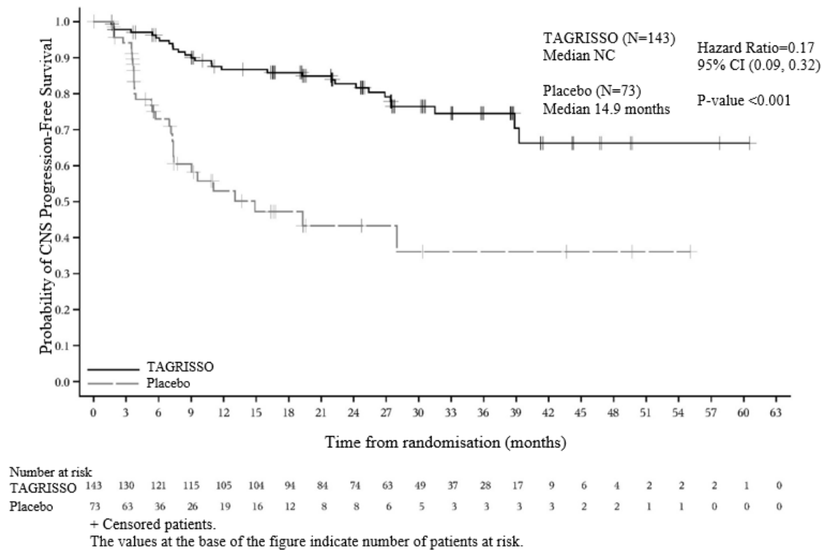
Figure 4 Kaplan-Meier Curves of CNS PFS as assessed by BICR in LAURA
