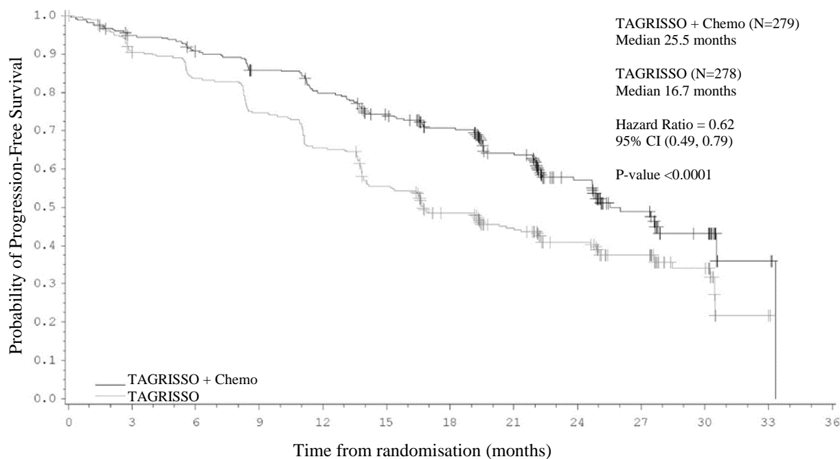
Figure 7 Kaplan-Meier Curves of Progression-Free Survival as assessed by investigator in FLAURA2
