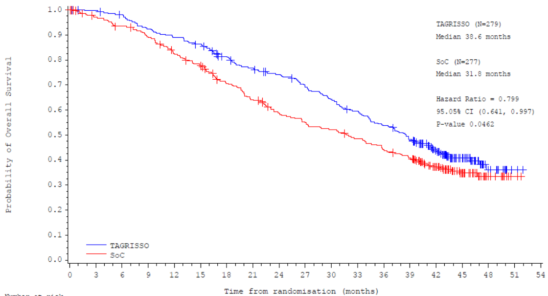
Figure 6 Kaplan-Meier curves of overall survival in FLAURA
